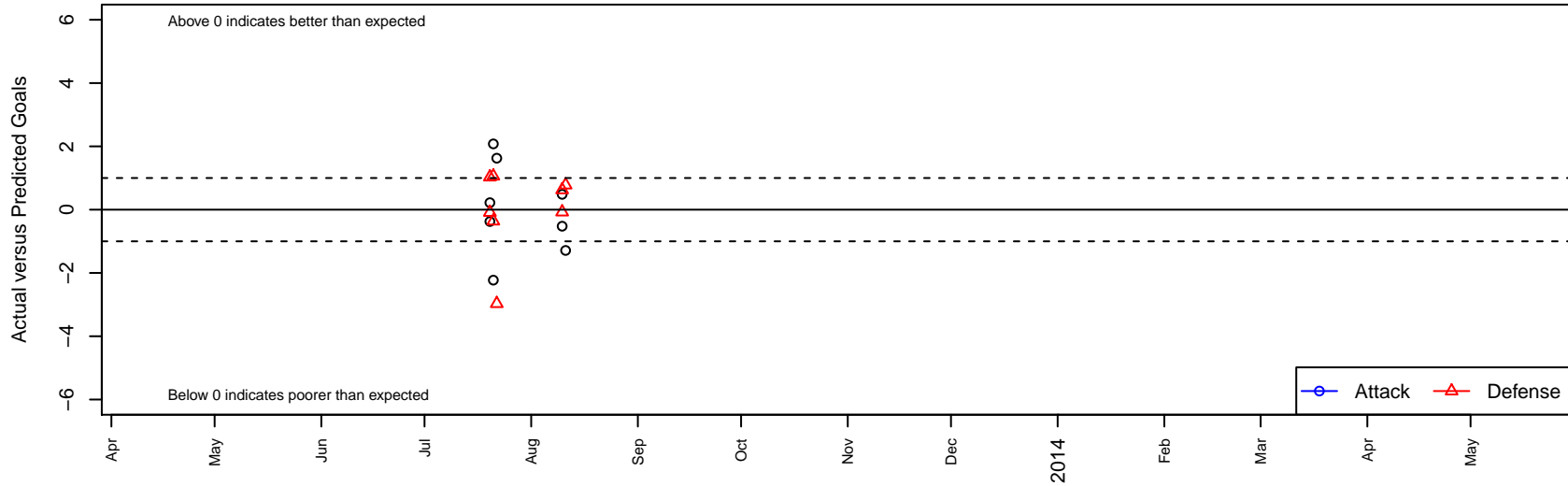
Chivas Guadalajara SA B96 Dots are actual minus expected GF (blue circles) and GA (red triangles). Blue line is smoothed change in attack strength. Red is smoothed change in defense strength.
